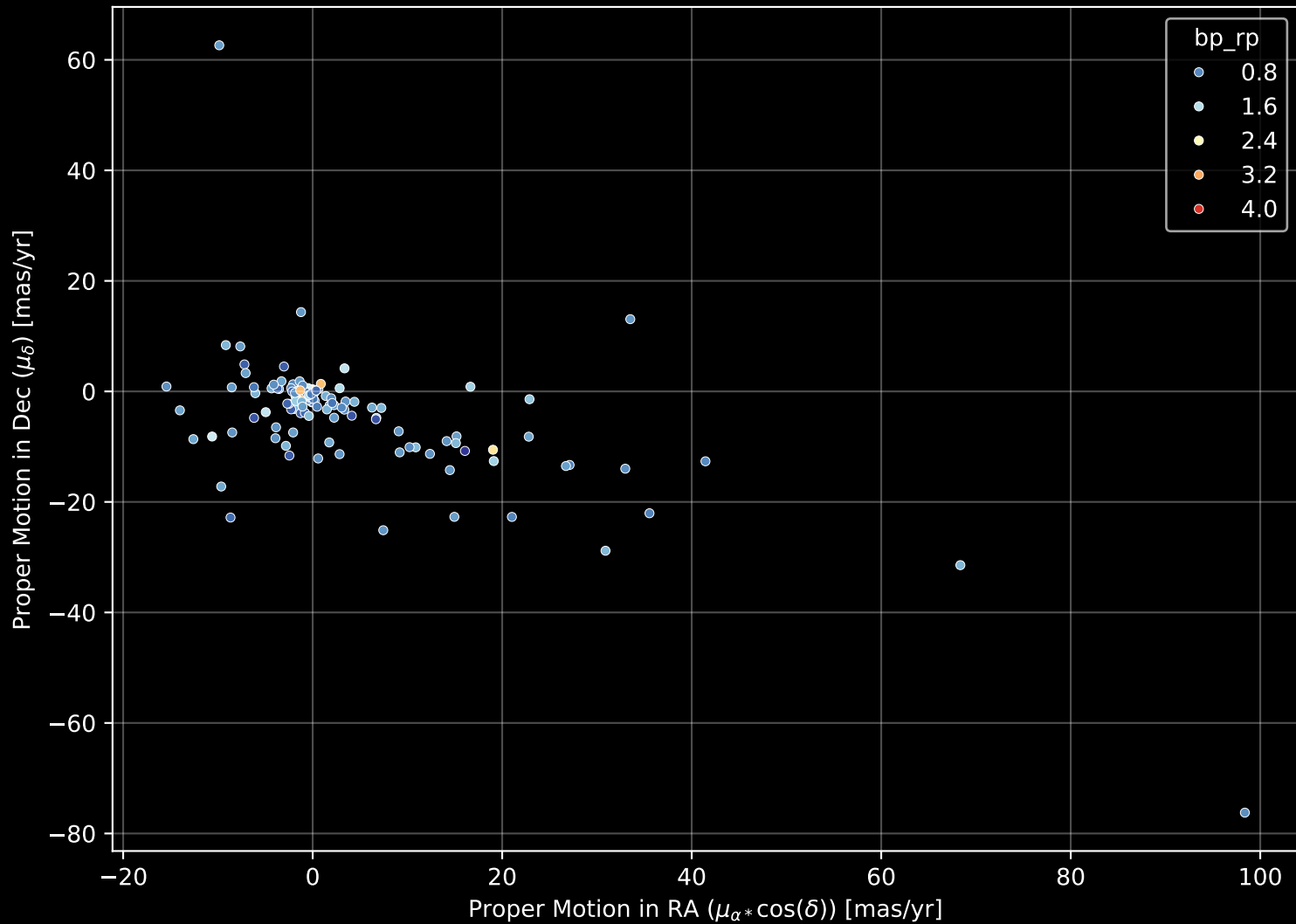
APOGEE DR17 Field: [W3-4] Proper Motion Diagram (n= 193)
