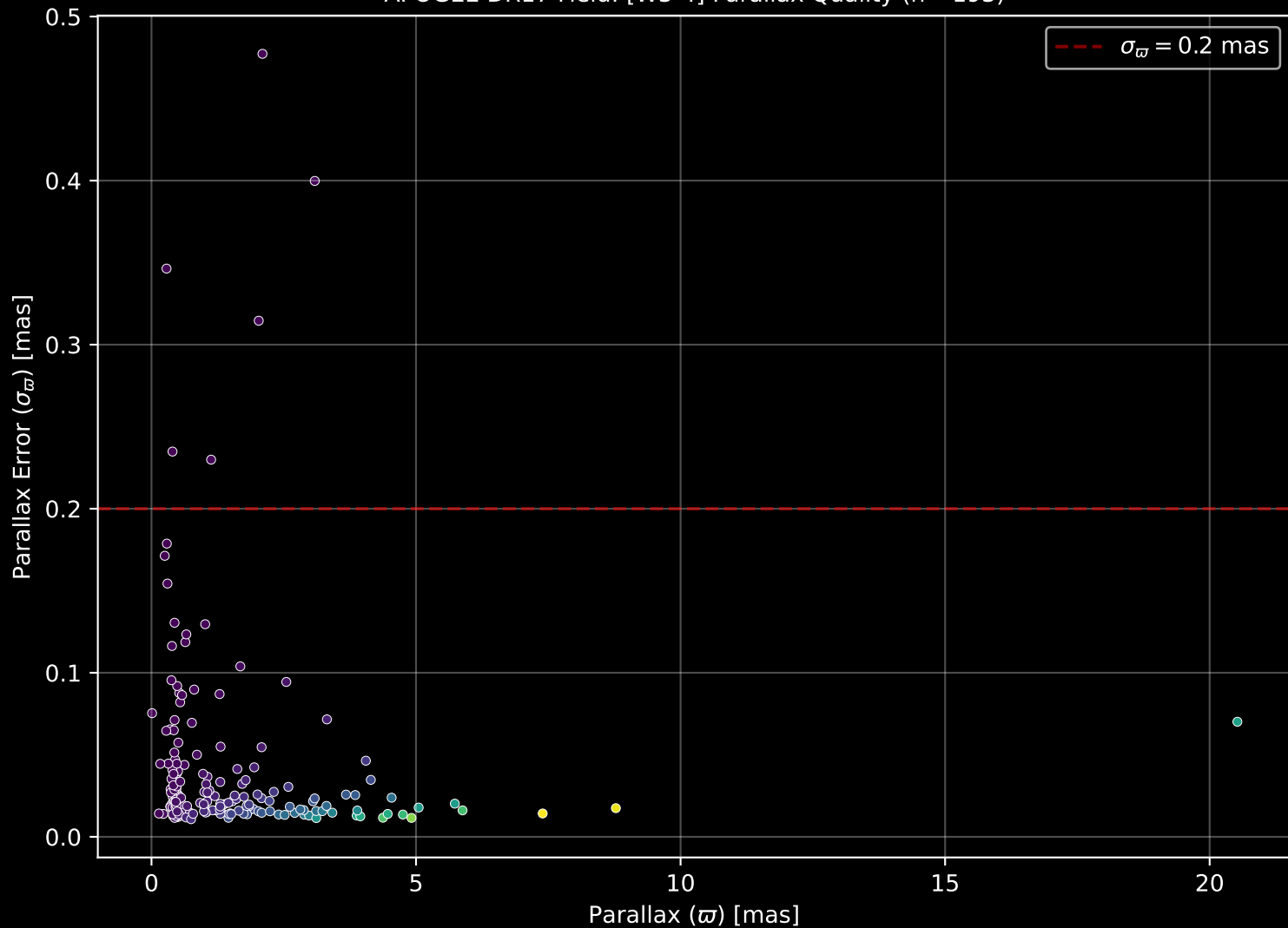
APOGEE DR17 Field: [W3-4] Parallax Quality (n= 193)
