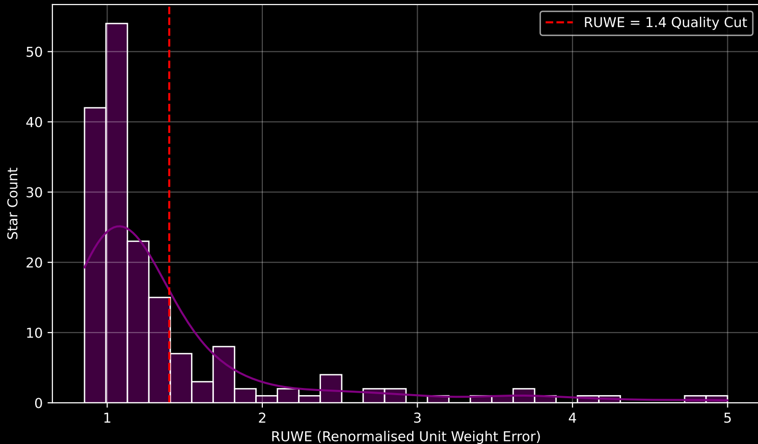
GAPOGEE DR17 Field [W3-4] RUWE Distribution (n= 176)
